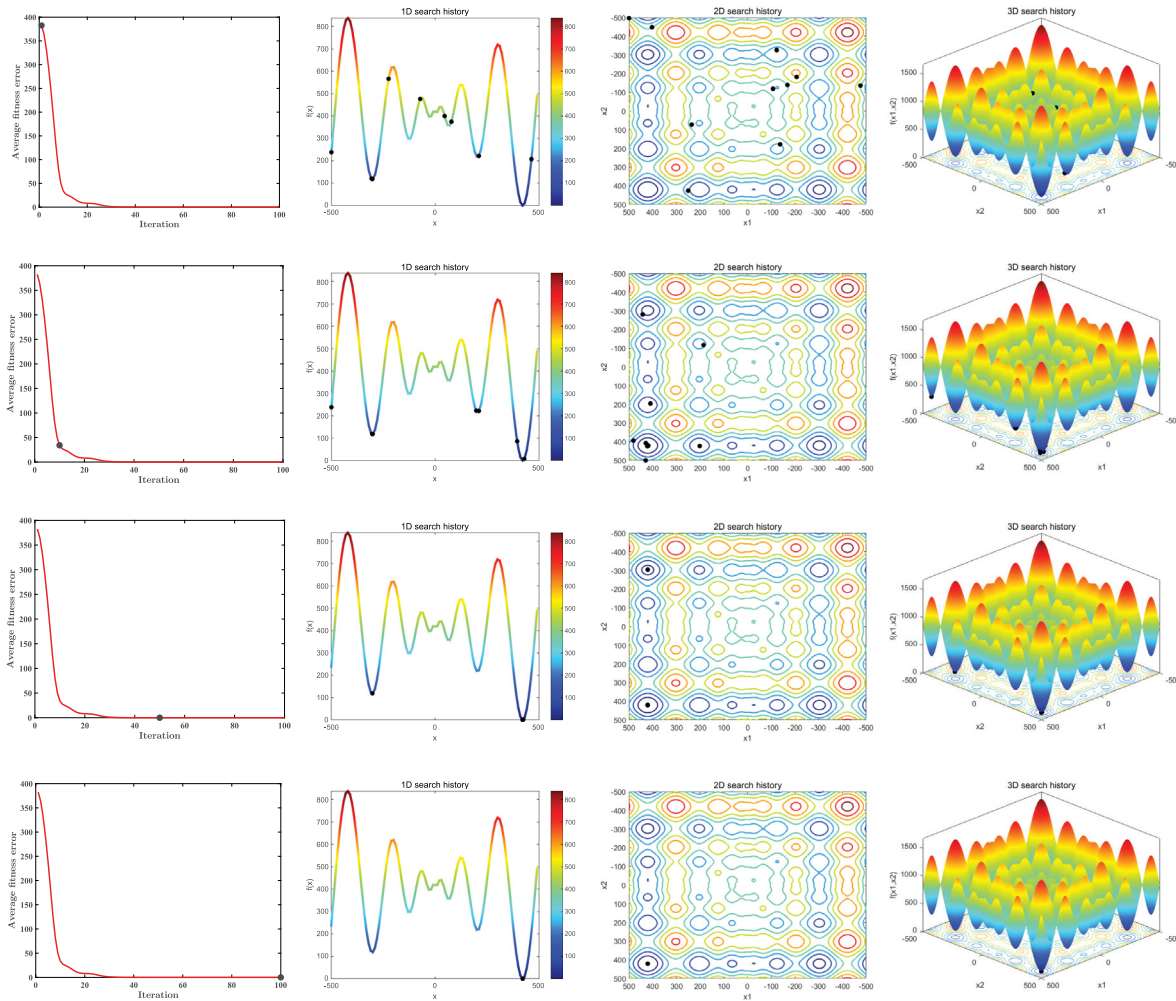
Fig. 3. Qualitative metrics: average fitness error, 1D search history, 2D search history, and 3D search history.
