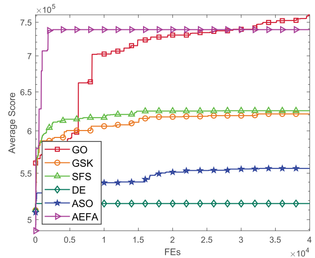
Fig. 9. The algorithm obtains an average score for the quality of the aligned sequences during HMM training.
