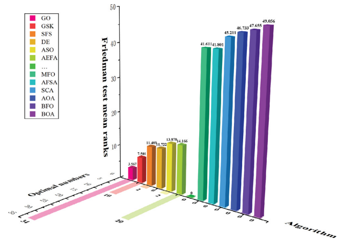
Fig. 6. The Friedman test mean ranks and the optimal numbers for better and worse algorithms.
