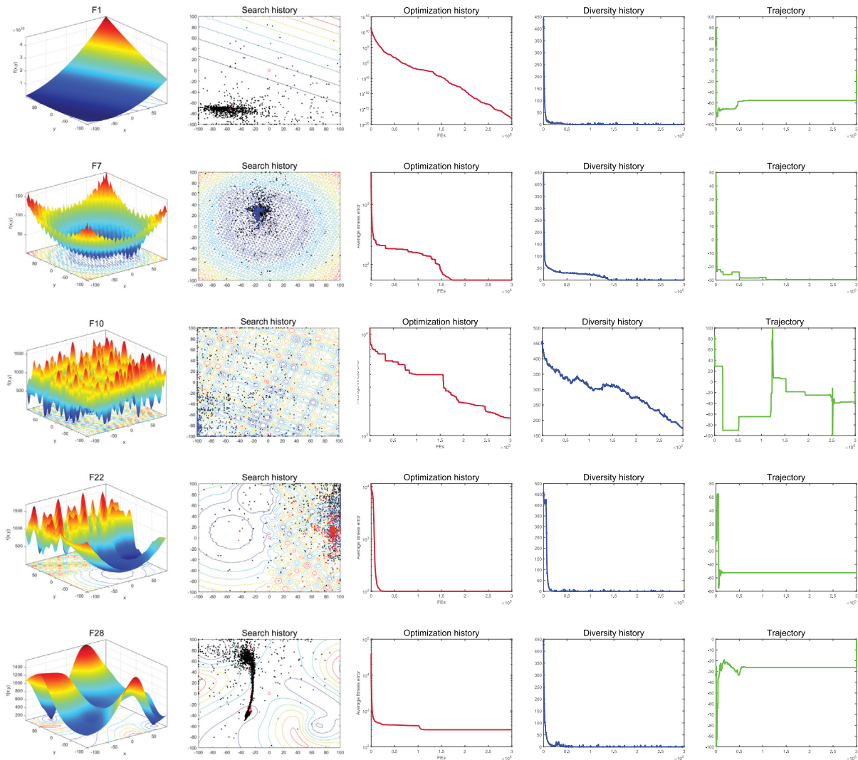
Fig. 7. Qualitative metrics: search history, optimization history, diversity history, and trajectory.
