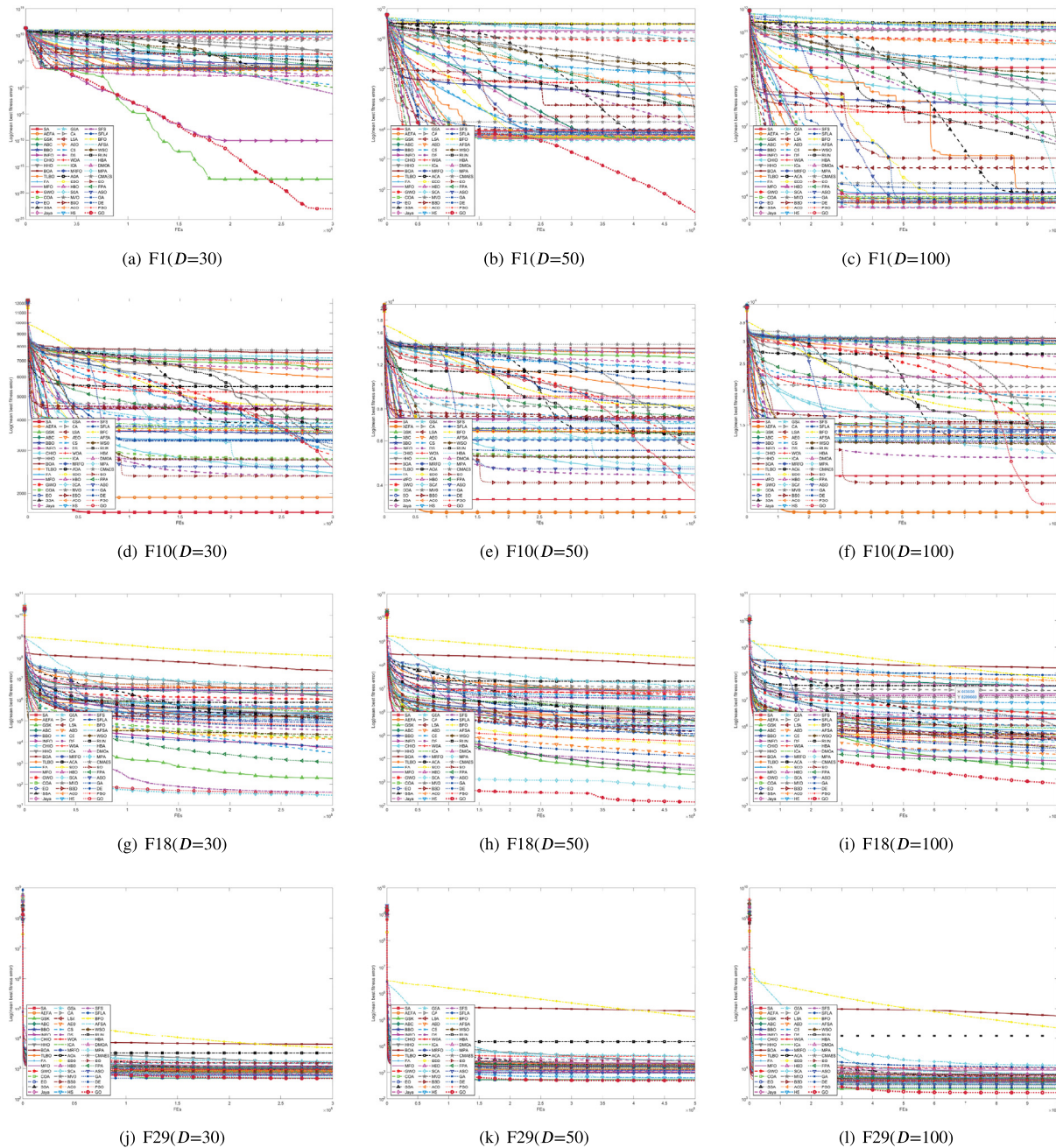
Fig. 4. The convergence curves of GO and the other 50 metaheuristic algorithms on four groups of problems.
