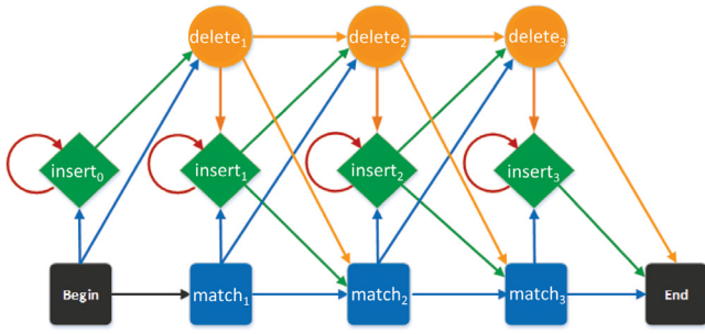
Fig. 8. Example of profile HMM of length 3 for the MSA problem.
